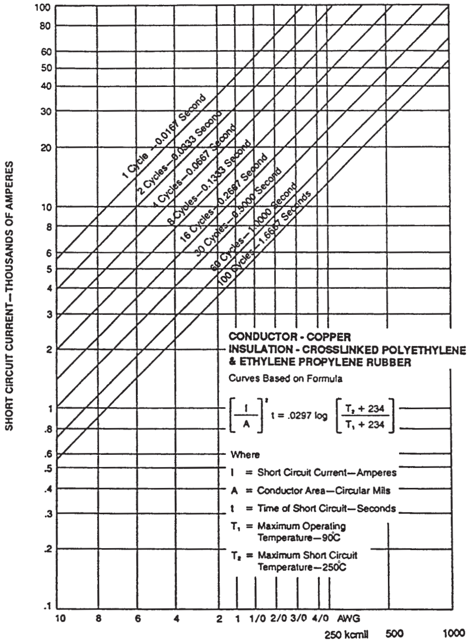
Copper Correction Factors for Various Short Circuit Temperatures:
